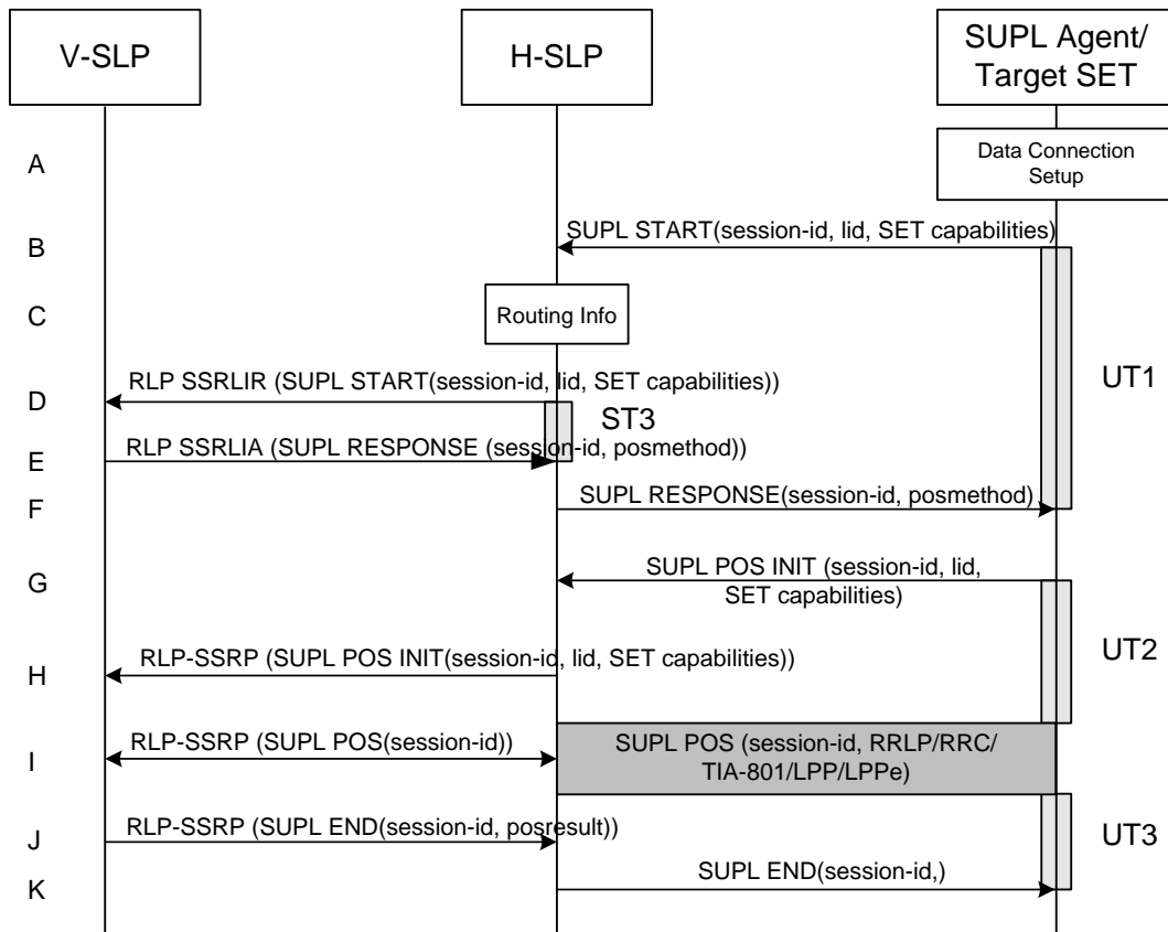
Figure 48: SET-Initiated Roaming with V-SLP Positioning Successful Case – Proxy mode
