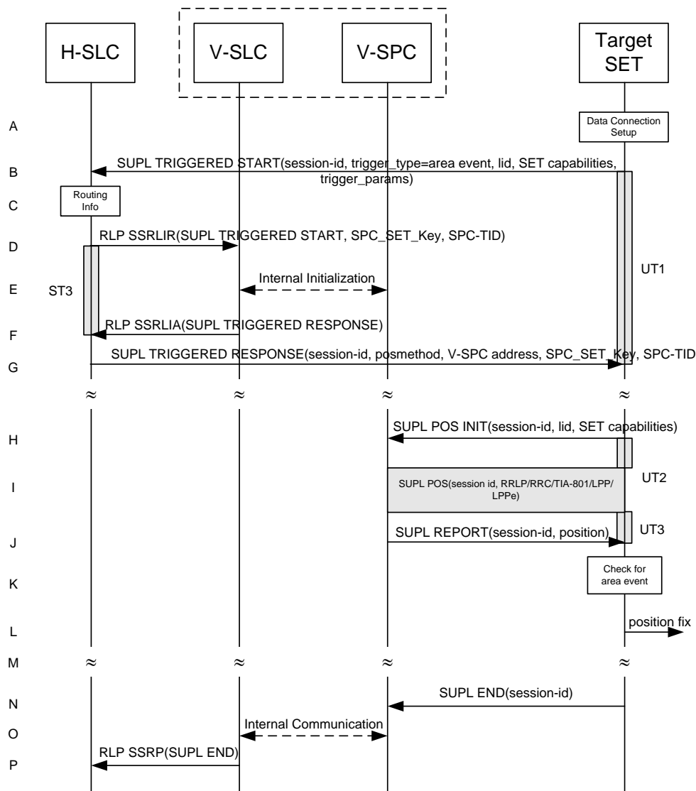
Figure 63: SET Initiated Area Event Trigger Service Roaming with V-SLP Positioning Successful Case – Non-Proxy Mode
