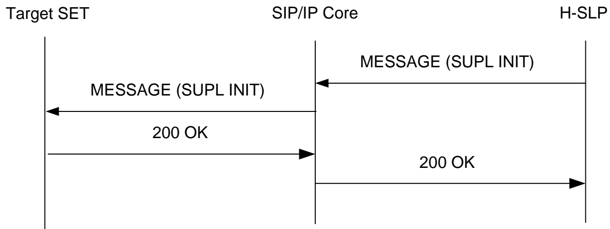
Figure 87: SIP Push Message flow
