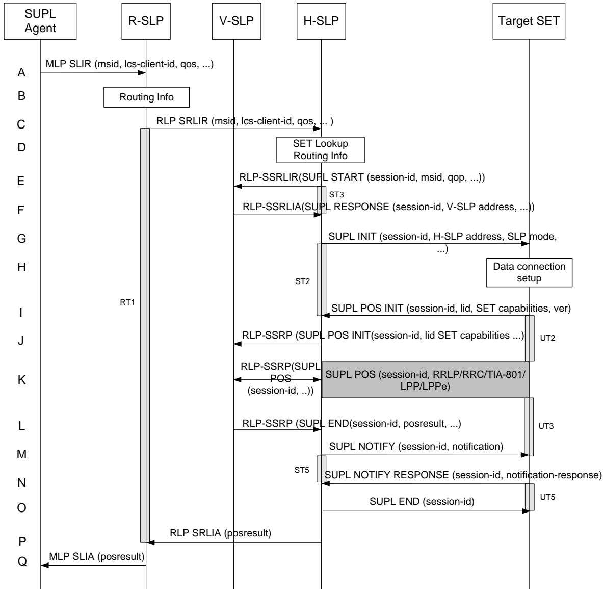
Figure 23: Notification/Verification based on current location. Network Initiated Roaming with V-SLP Positioning Successful Case – Proxy mode
